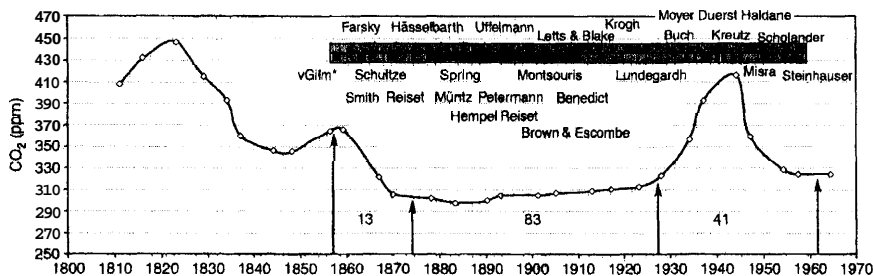
Fig. 10. Local CO 2 concentrations in northern hemisphere from 1812–1961 by chemical assay. Data smoothed by use of 11-year average. Numbers between vertical arrows show number of measurement campaigns. Important analysts with time period of assays are shown in dark gray and black. Adapted from Beck (2007).
