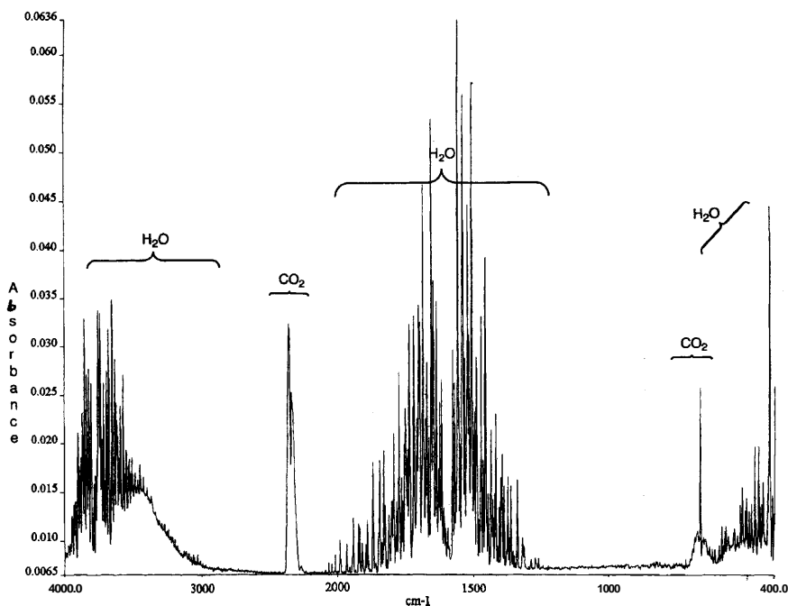
Fig. 7. Infrared spectrum of air at sea level, 760 torr, 28°, relative humidity 76%, 29 June 1999. Absorbance vs. frequency in wavenumbers ( \text{cm}^{-1} ) corresponding to wavelengths of 2.5–25 \mu\text{m} . Other experimental details in Kauffman (2004). Used with permission from The Journal of Chemical Education .
