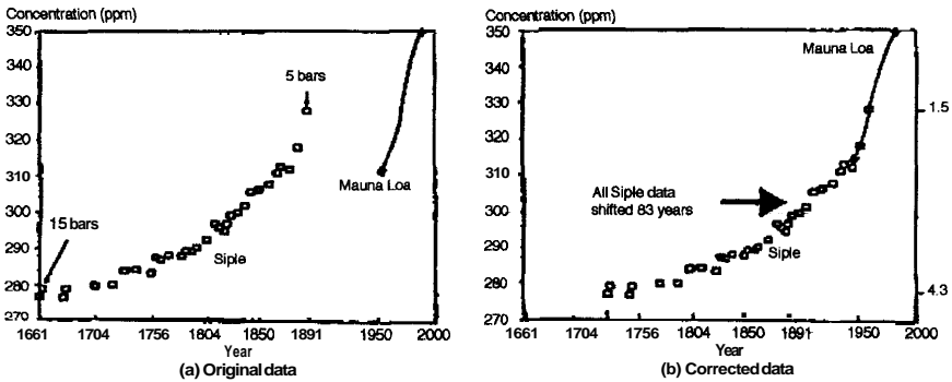
Fig. 9. Altering the ice core data (open squares) to fit the AGW Hypothesis. Solid line is \text{CO}_2 concentration in ppm in atmosphere from Mauna Loa. Original data in (a), arbitrary "correction" of 83 years in (b). Adapted from Jaworowski (1997, 2007).
