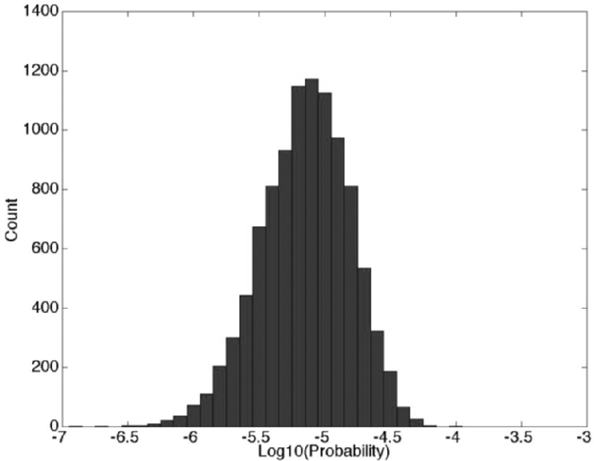
Fig. 1. Histogram of \log_{10}(\text{Probability}) found from Rule of Succession estimates derived from 10,000 Monte Carlo simulations of the dataset shown in Table 3.
