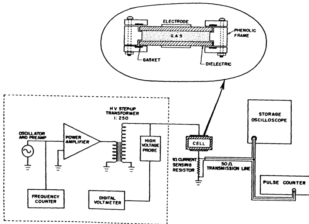
Fig. 3. Schematic of system: Detector, power supply and monitoring system for counting mode and oscilloscope mode. Equipment: Oscillator and preamp custom made (precision); power amplifier—Crown DC 300 A; H.V. step-up transformer—custom made; H.V. Probe—Tektronix P-6015; frequency counter—Fluke 1900 A; digital voltmeter—Fluke 8600 A (4 digit); storage oscilloscope—Tektronix 7834; counter—Hewlett Packard 5328 A.
