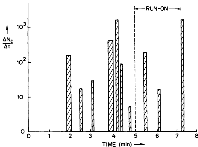
Fig. 6. Schematic illustration of counting rate, \Delta N_c/\Delta t , as a function of time during a five-minute WBH period and the run-on period.
