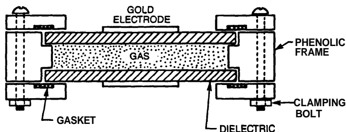
Fig. 1. Schematic of detector cross-section.
