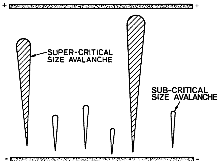
Fig. 5. Illustration of subcritical and supercritical electron avalanche relative size for counting purposes.
