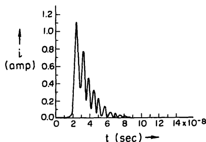
Fig. 4. Typical oscilloscope trace of electron avalanche current vs time; 200 mA/vertical division and 10^{-8} sec/horizontal division.
